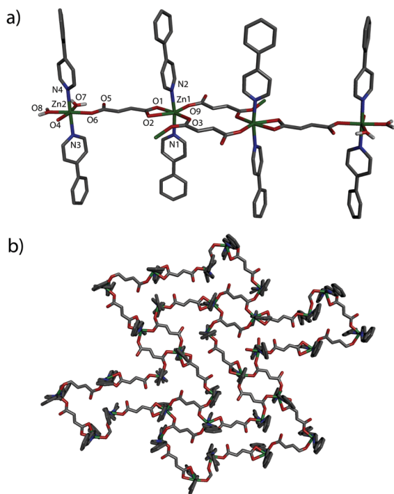
Fig. 1 (a) Basic structural unit showing the coordination environment around the metal centres. (b) A part of 2D structural network showing the 4.8^2\text{-fes} framework. H-atoms are not shown for clarity.
