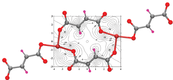
Fig. 3 Variation of NICS(0) over the surface of the 14-membered metal ligand ring.
