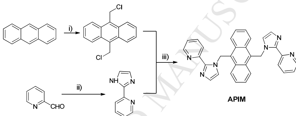
Scheme 1: Reagent and conditions: i) Paraformaldehyde, Anh. \text{ZnCl}_2 , Conc. \text{HCl} , 1,4-Dioxane ii) 40% Glyoxal, Conc. \text{NH}_3 , stirring, 1h, 0^\circ\text{C} , iii) \text{NaOH} , \text{PhCl}/\text{H}_2\text{O} , \text{Bu}_4\text{NBr} , reflux.
