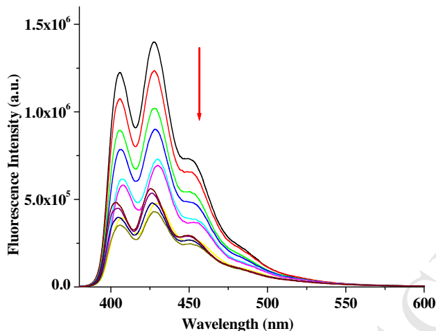
Fig. 8. Change in emission spectra of APIM ( c = 2.5 \times 10^{-5} M) upon addition of Zn^{2+} ( c = 1.00 \times 10^{-3} M, as perchlorate salt) in CH_3CN ( \lambda_{ex} = 370 nm).
